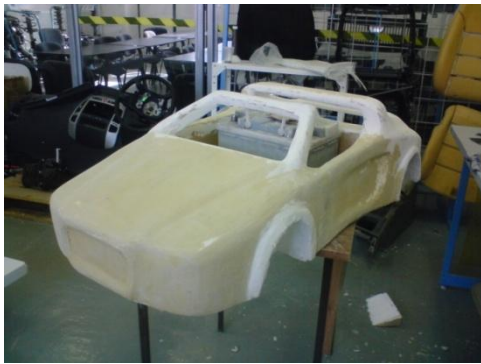
Fig. 5: Mockup fabrication (scale 1:4)
